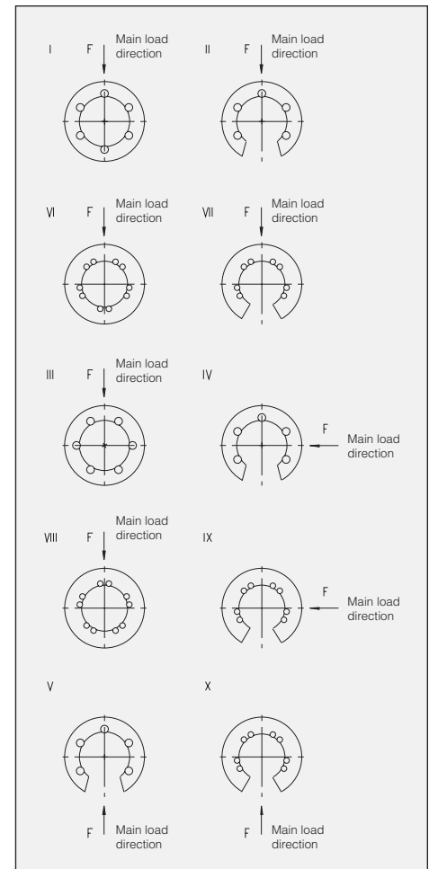
Figure 2 Load Cases
