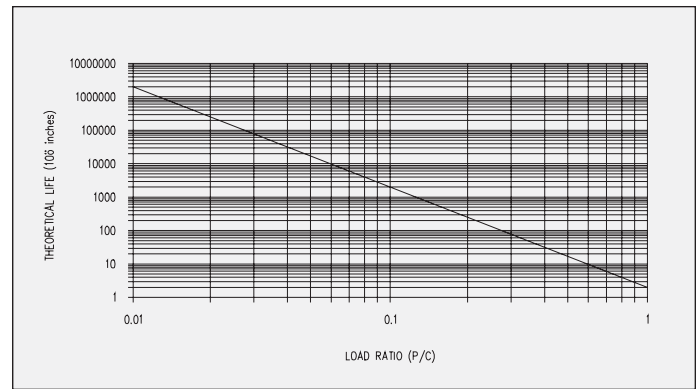
Theoretical Life
